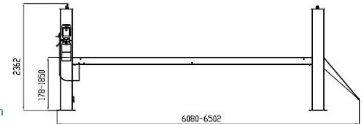
Front extension kit for option
